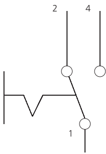
NZK2-32/1
